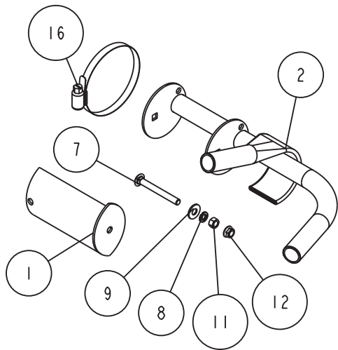
DETAIL A SCALE 0.125
