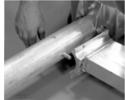
6. Mount the guide post tube (Ref.#9) to the opposite end of the lower frame weldment using a leg adjustment pin (Ref.#10). Secure with a hitch pin clip (Ref.#45).
