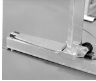
8. Slide the platform assembly (Ref.#18) into the winch post extrusion (Ref.#14) as shown.
