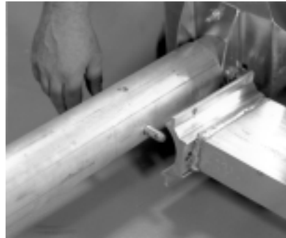
5. Mount the guide post tube (Ref.#9) to the opposite end of the lower frame weldment using a leg adjustment pin (Ref.#10). Secure with a hitch pin clip (Ref.#43).
