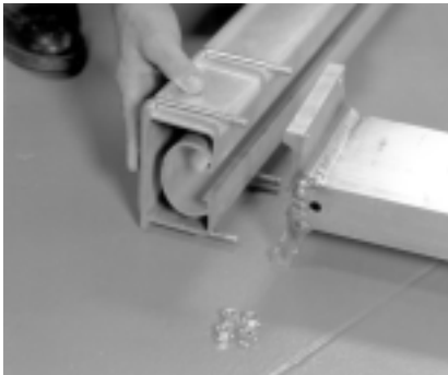
4. Mount the lower frame weldment (Ref.#6) to the winch post extrusion (Ref.#14) using two (2) 3/8" X 5-3/16" X 3-7/8" square u-bolts (Ref.#28) as shown. Secure with 3/8" flange lock nuts.
