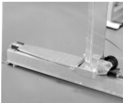
7. Slide the platform assembly into the winch post extrusion (Ref.#14) as shown.
