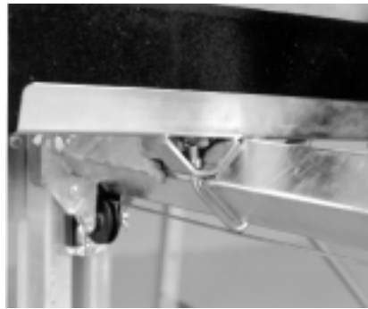
21. Mount the bunk with brackets onto the platform weldment using two (2) 1/2" v-shaped u-bolts (Ref.#30), two (2) spacers (Ref.#49) and two (2) 1/2" hex lock nuts per bunk as shown. Note: The short end of bunk from galvanized mounting channel goes to the right of the winch handle (as reference - Refer to picture 22 for Right and Left of hoist). Repeat on other bunks. Bunks should be spaced to fit your watercraft before tightening. Bunks should also be angled toward the center of the platform. NOTE: To enter the dock hoist from the other end - reverse the bunk assembly.
